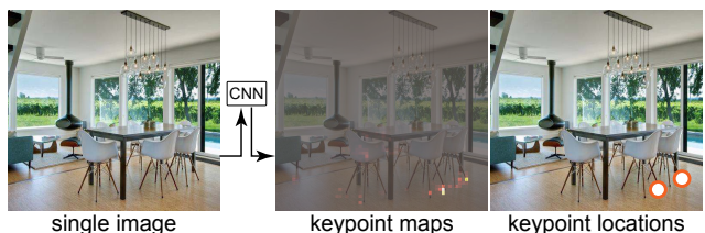
Figure 3: We trained a neural network on real images to detect keypoint maps , which are then converted to 2D keypoint locations via thresholding and non-maximal suppression.
