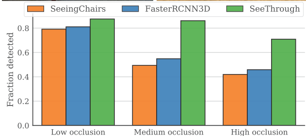
Figure 1: We present SEETHROUGH, a method to detect objects (specifically chairs) from single images under medium to heavy occlusion by reasoning with 3D scene-level context information. Our method significantly improves detection rate over state-of-the-art alternatives.
