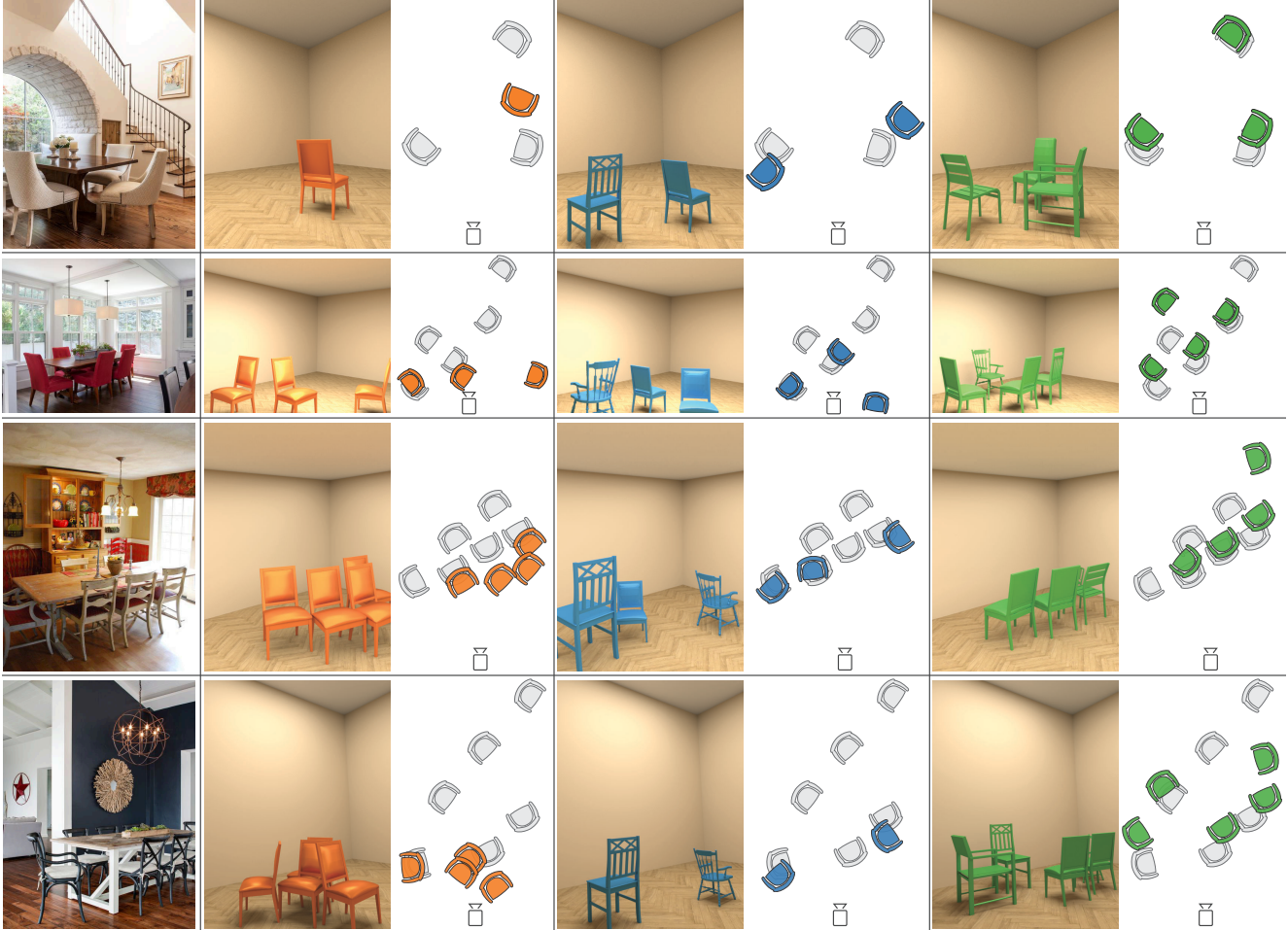
Figure 5: Qualitative comparison of the baseline methods: SEEINGCHAIRS (orange) and FASTERRCNN3D (blue) against SEETHROUGH (green). Annotated groundtruth poses (gray) are provided for reference in the top view. Note that our approach both detects more chairs and correctly aligns them compared to the others.
