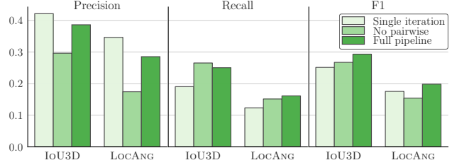
Figure 8: Ablation study evaluating the importance of the different stages of SEETHROUGH.
