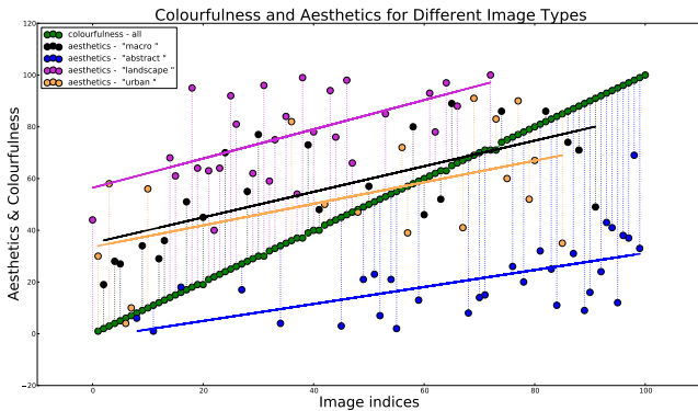
Figure 8: Colourfulness vs. aesthetics for different image types: “landscape”, “abstract”, “macro” and “urban”.
